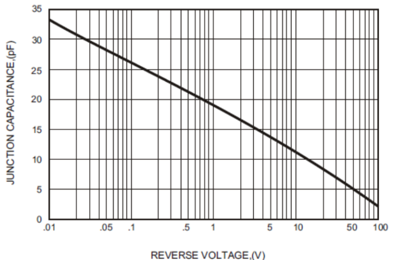
FIG.5-TYPICAL JUNCTION CAPACITANCE
