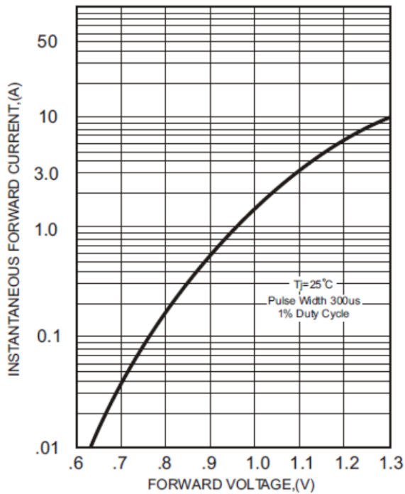
FIG.1-TYPICAL FORWARD CHARACTERISTICS
