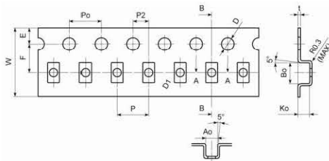
▲ Embossed taping dimension
