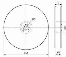
▲ Tape/Reel dimension
